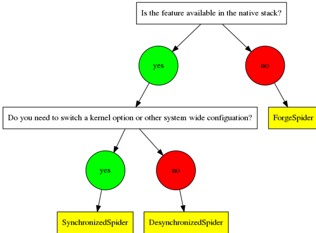
Fig. 1.2: A flowchart to help choosing a model for your plugin
